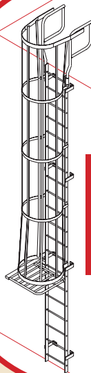
ACC 20BRC Steel Access Ladder with Boarding Rails, Cage and Bottom Hoop Security Hatch
