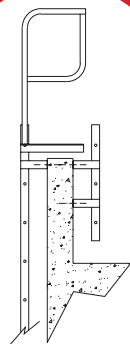
Typical Roof Parapet Application: Outside Ladder has Boarding Rails and Upper Platform
